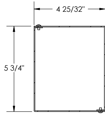
SECTION C-C SCALE 1 : 4
