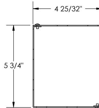
SECTION C-C SCALE 1 : 4
